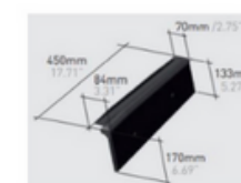
Q88 PLANUM RIGHT SIDE CLOAK VERGE
