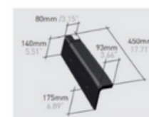
Q89 PLANUM LEFT SIDE CLOAK VERGE
